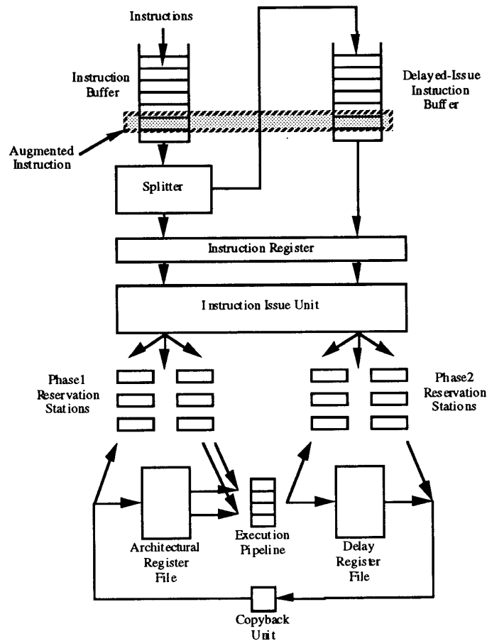
Figure 3. Processor organization for supporting split-issue with out-of-order execution.
