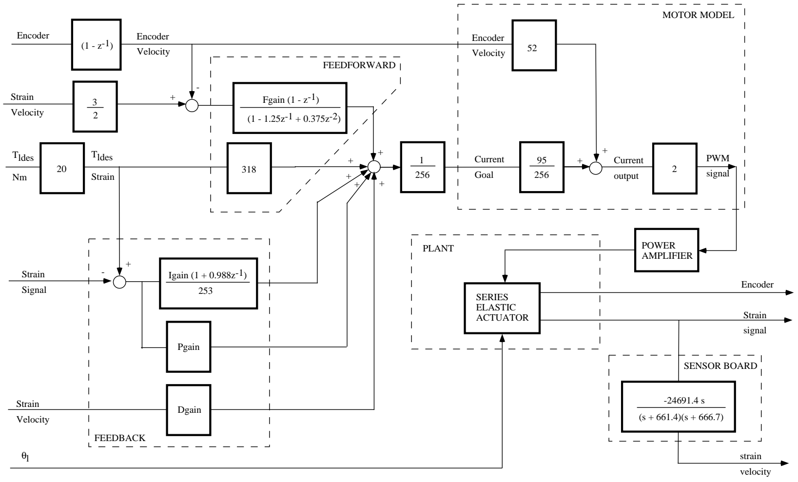
Figure 5-17: The control system
