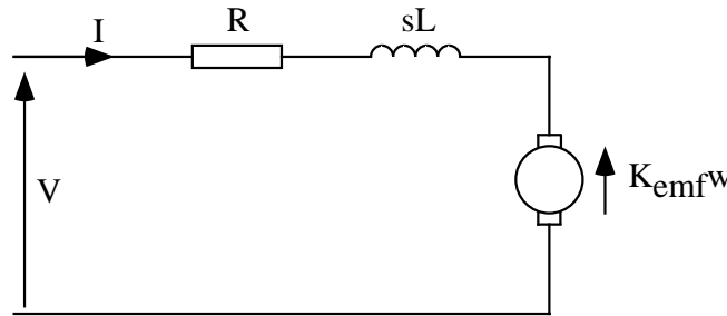
Figure 4-8: Motor model
