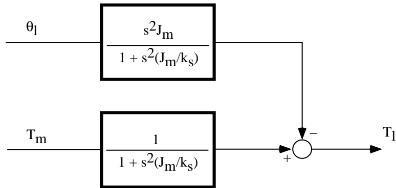
Figure 3-2: Plant model
