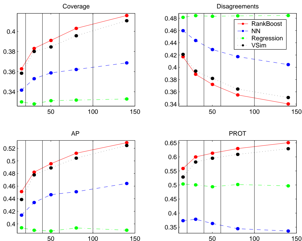
Figure 6: Performance of the algorithms on different feature densities.
