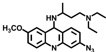
Quinacrine Azide
