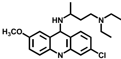
Quinacrine
