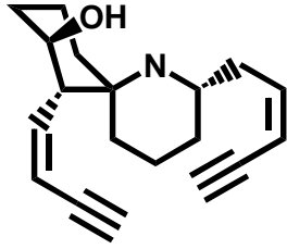
Histronicotoxin (HTX)
