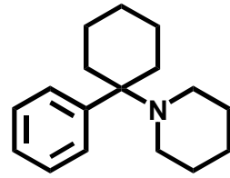
Phencyclidine (PCP)
