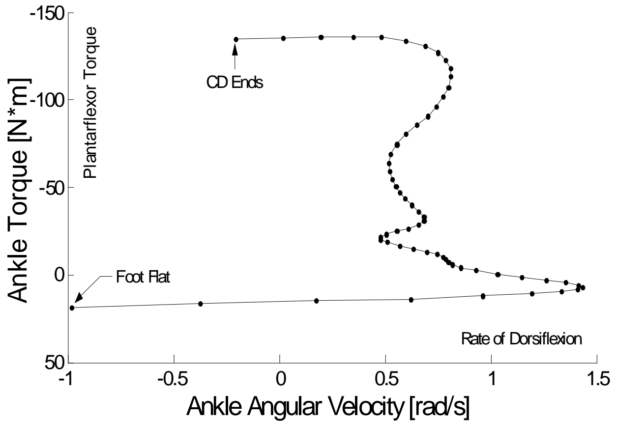
Figure 3.4 Scatter plot of ankle torque versus ankle angular velocity during controlled dorsiflexion (CD). Data shown are from a single trial of subject FJI walking at the self-selected normal gait speed and are representative of the subject's trials. Data points are equally spaced in time.
