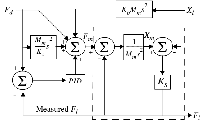
Fig. 6. Control Architecture
