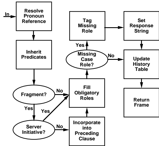
Figure 2: Block diagram of flow control in discourse module.
