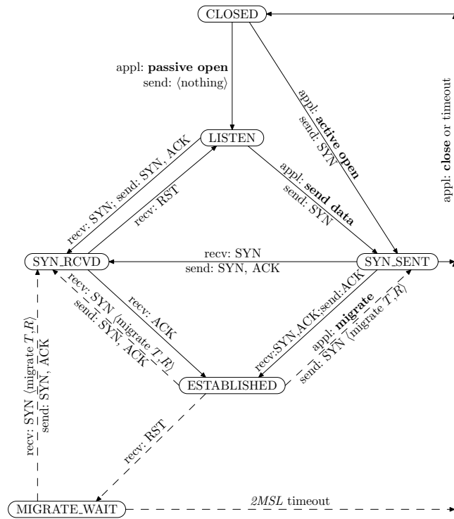
Fig. 4. Partial TCP state transition diagram with Migrate transitions (adapted from [34, figure 18.12])
