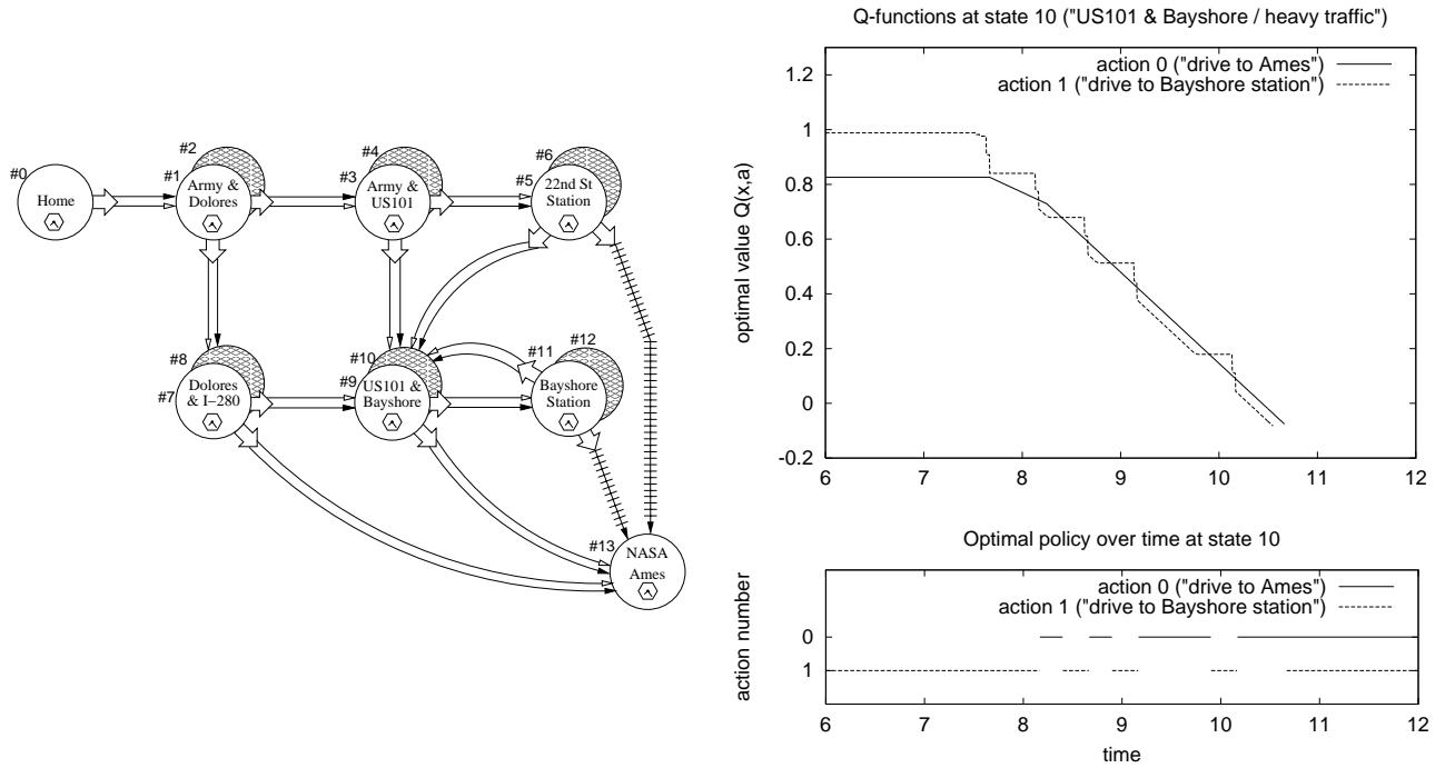
Figure 1: The San Francisco to Ames commuting example. At right, the optimal value function and policy at location 10.
