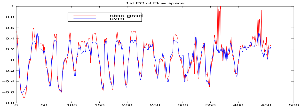
Figure 1: Estimates of LMM flow parameter using the stochastic gradient descent and support vector regression on a test sequence of 459 images.
