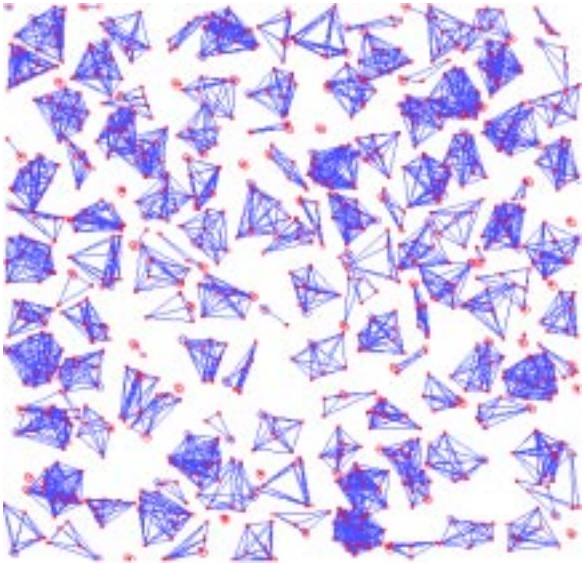
Figure 9: Result of the first phase of the tight club algorithm.
